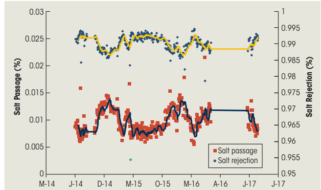
Train A Normalized Salt Passage and Rejection during 940 days of operation
